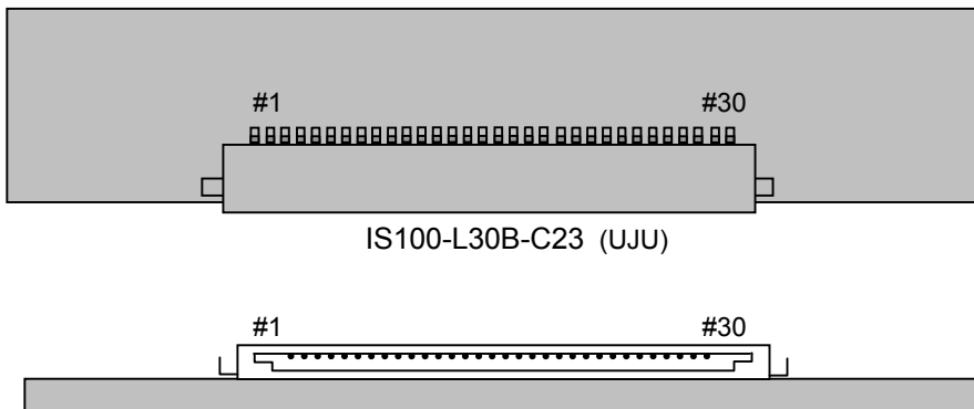
Rear view of LCM
