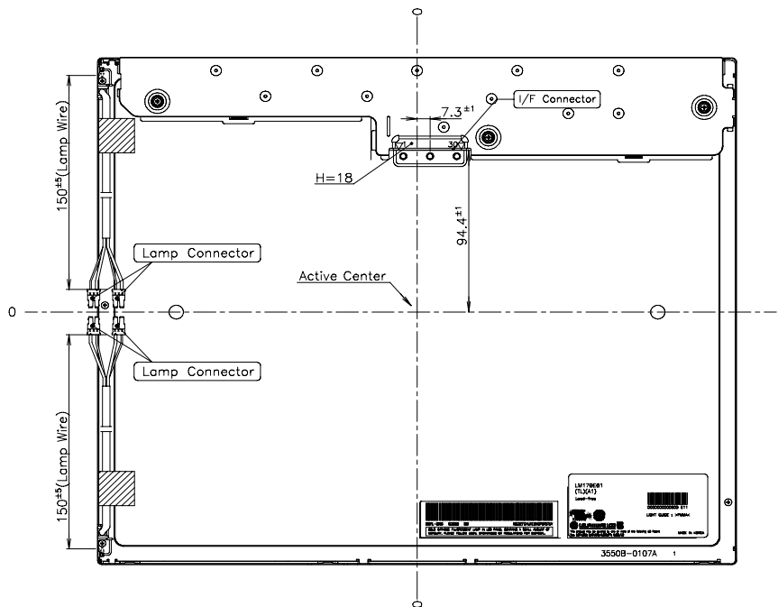
Figure 15. Rear view
