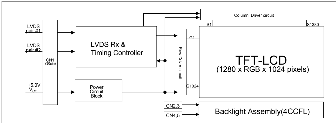
Figure 1. Block diagram
