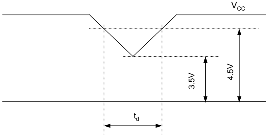
[ Figure 8 ] Power dip condition
