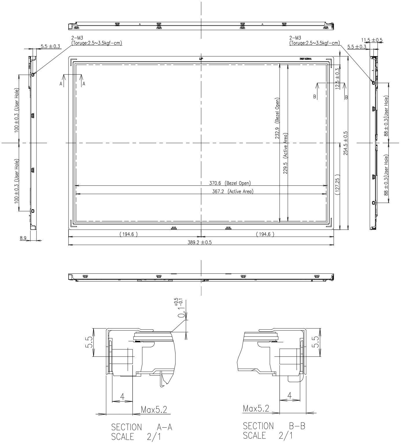
Figure 14. Front view
