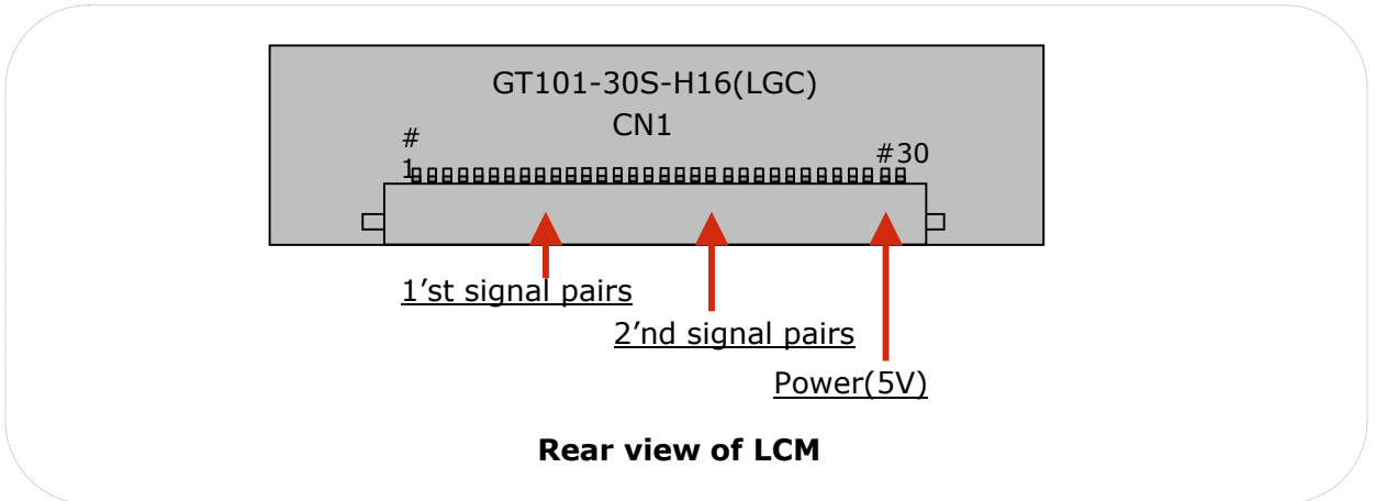
FIG. 4 Connector diagram
