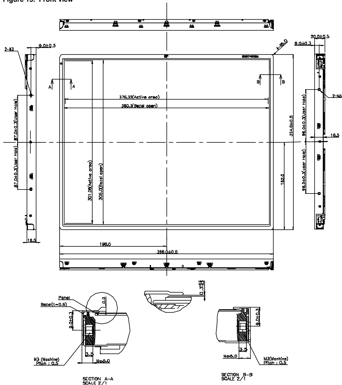
Figure 15. Front view
