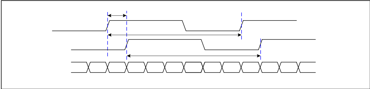
< Clock skew margin between channel > t_{SKEW\_EO}
