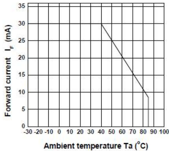
Diode IF-Ta CHARACTERISTICS DIAGRAM
