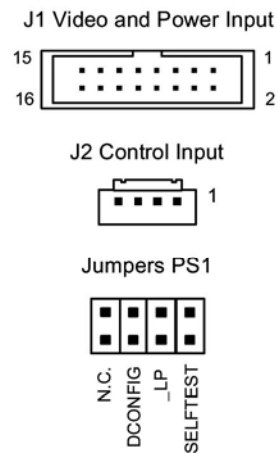
Fig 2. Input Connectors and Programmable Jumpers.
