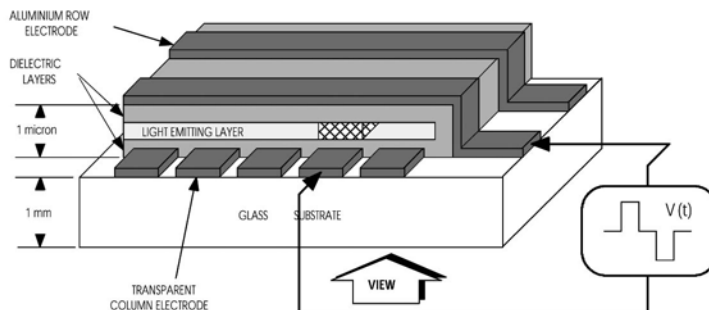
Figure 1. EL Technology.
