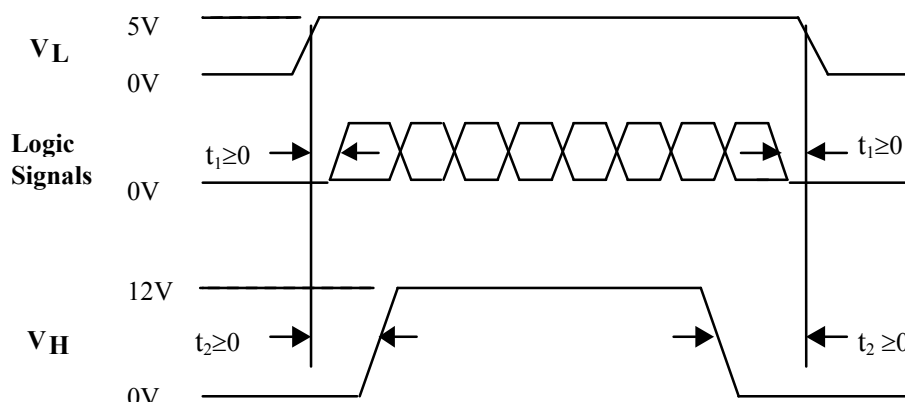
Figure 1. Data/Power Connector
