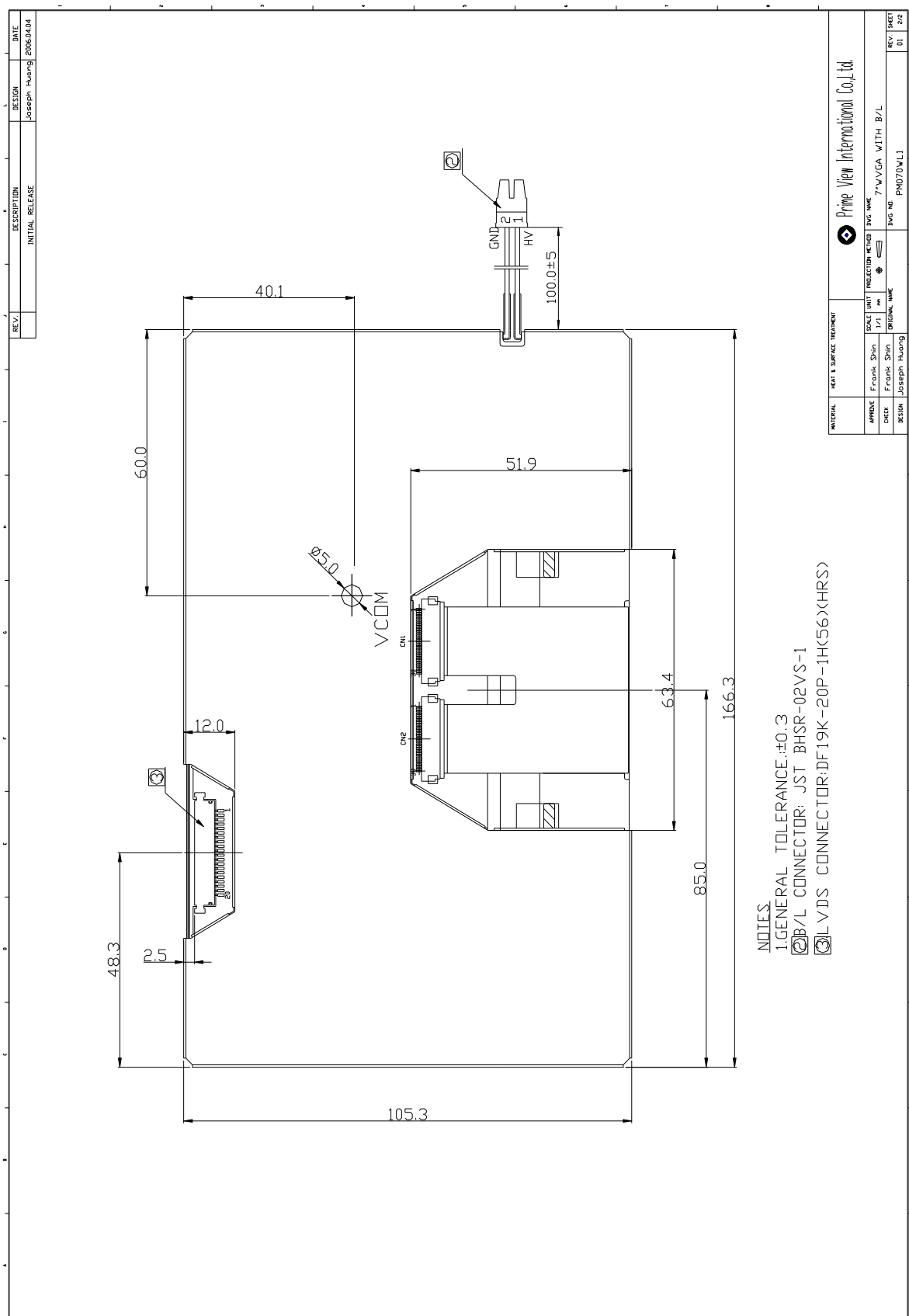
Outline Drawing : Rear View (unit mm)
