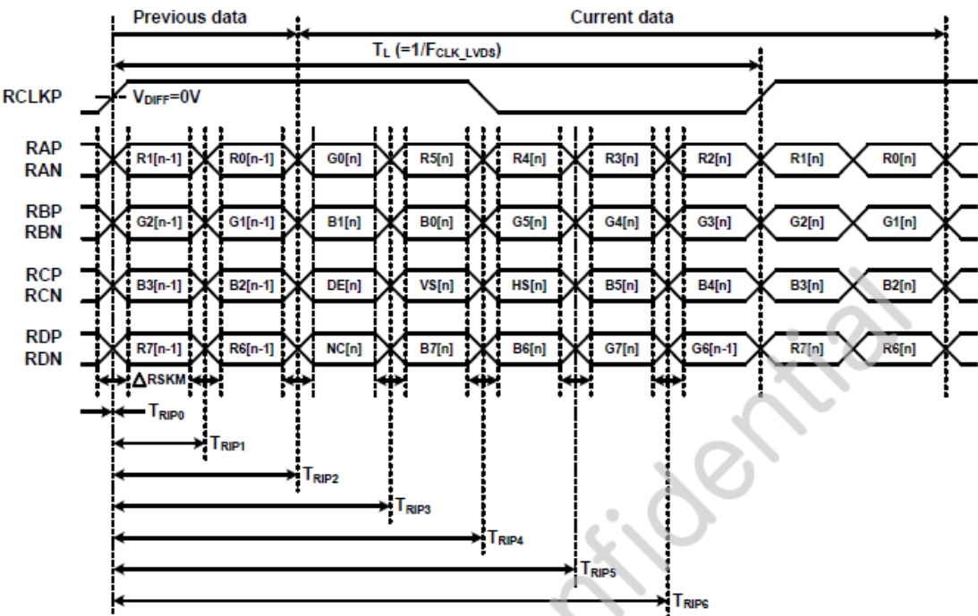
Note (2) : LVDS Input Timing Diagram
