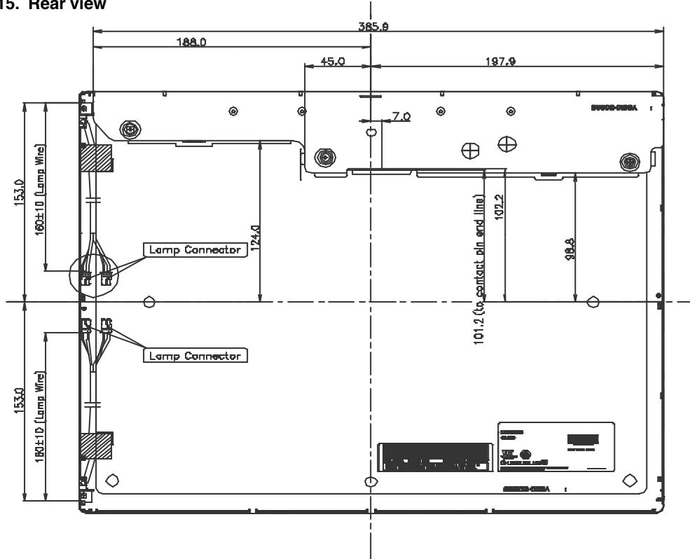
Figure 15. Rear view
