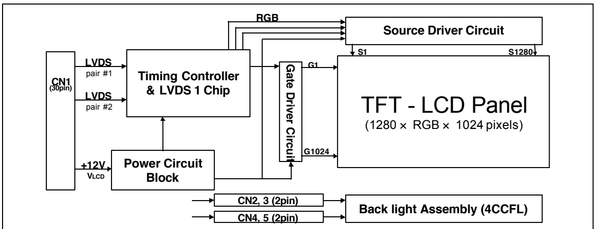
Figure 1. Block diagram
