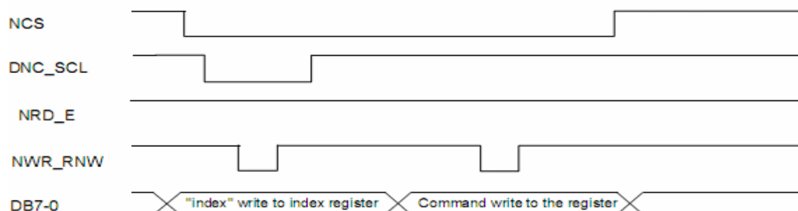
Figure 5.1 Register write timing in parallel bus system interface (for I80 series MPU)
