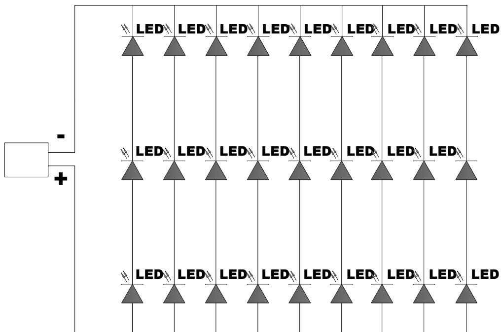
Figure 3.1 LED driver circuit
