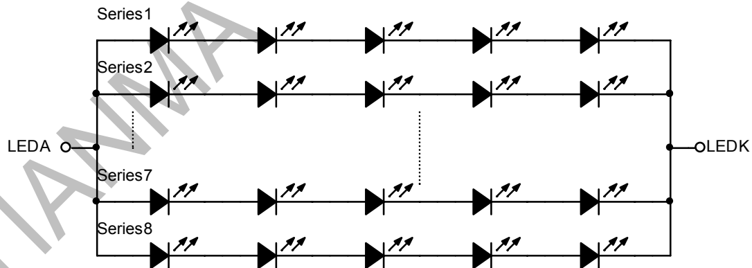
Figure 2.4 LED connection of backlight
