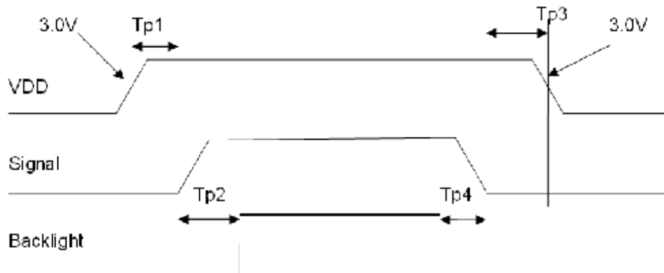
Figure 5.2 Interface power on/off sequenc
