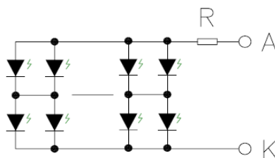
CIRCUIT DIAGRAM (LED 2X11=22 dies)
