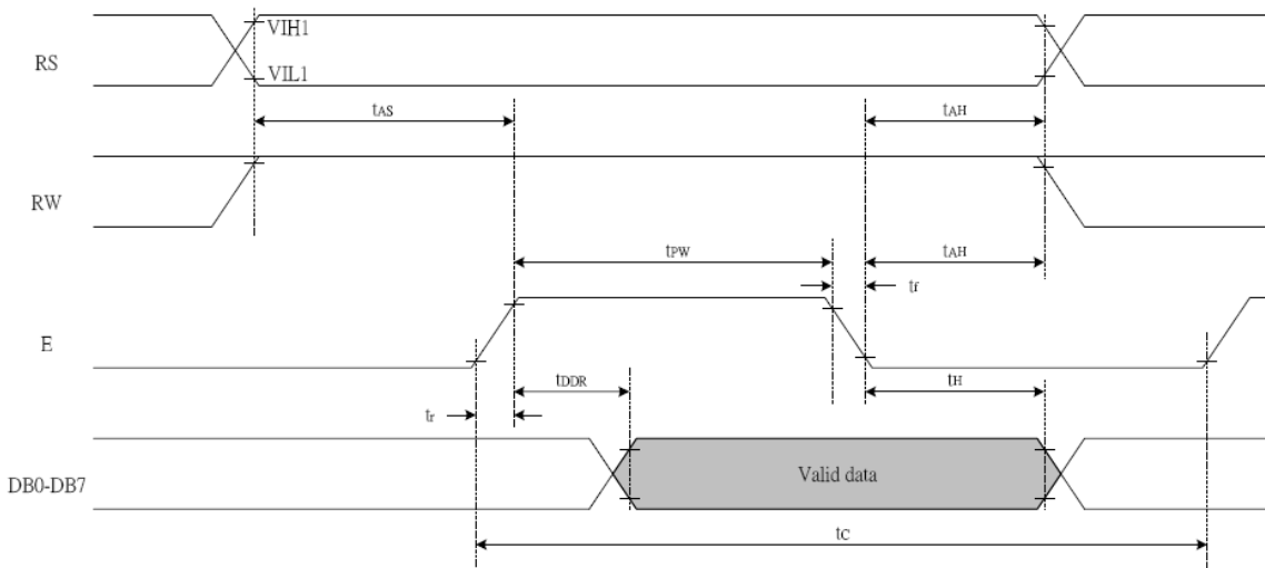
Figure2. Read Mode Timing Diagram
